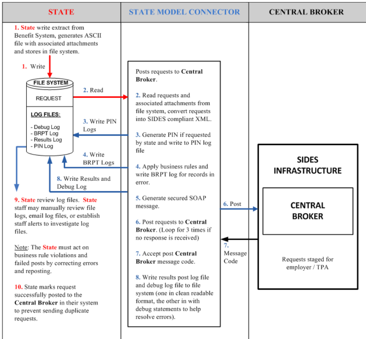
Figure 1. Model Connector Post for ASCII Files
